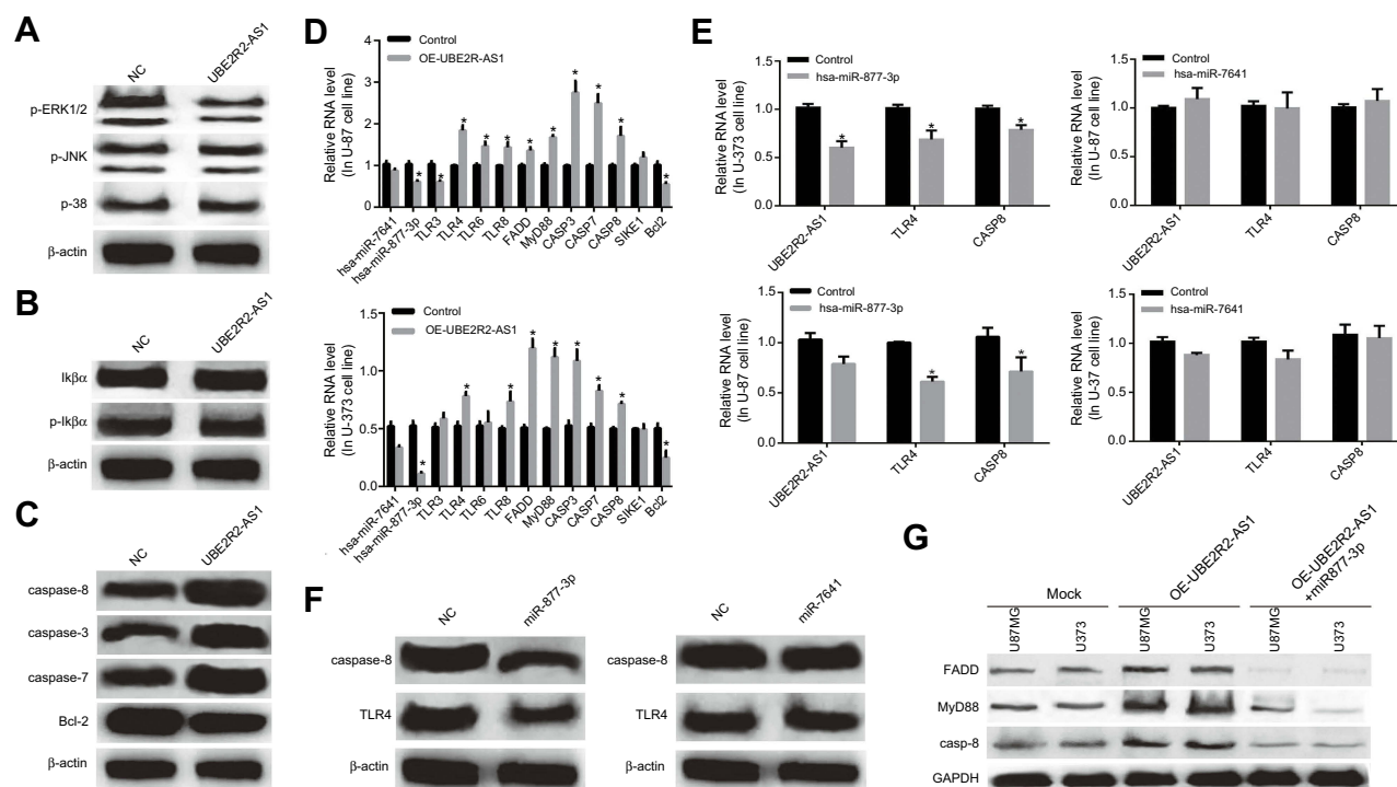
Figure 3 UBE2R2-AS1 and miR-877-3p inversely regulated cell apoptosis by Toll-like receptor signaling pathway in glioma. (A) Western blot analysis of p-ERK2/1, p-JNK, p-38 protein level in UBE2R2-AS1 overexpressed U87 cells, with β-actin as an endogenous reference. (B) Western blot analysis on IκBα and p-IκBα in UBE2R2-AS1 overexpressed U87 cells, with β-actin as an endogenous reference. (C) The expression level of apoptosis-related proteins was detected in UBE2R2-AS1 transfected U87 cells through western blotting. β-actin was used as an endogenous reference. (D) The expression of TLR-related genes and apoptosis-related genes was analyzed by qRT-PCR assay and GAPDH was used as an internal control. (* P < 0.05 .) (E) Relative RNA level of caspase-8 and TLR4 was detected in miR-877-3p or miR-7641 mimics transfected U87 and U373 cells through qRT-PCR assay. GAPDH was used as an internal control. (F) Western blot analysis on caspase-8 and TLR4 in U87 cells transfected miR-877-3p or miR-7641 mimics, with β-actin as an endogenous reference. (G) Western blot analysis of FADD, MyD88 and caspase-8 protein level following treatment of U87 cells and U373 cells with pcDNA3.1-UBE2R2-AS1 and miR-877-3p mimics. β-actin was used as control.
