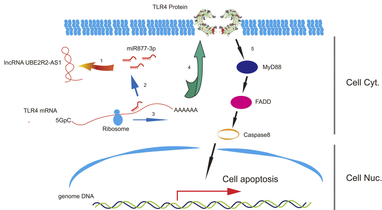
Figure 6 Molecular mechanism of the lncRNA UBE2R2-AS1. Step1 UBE2R2-AS1 takes sponging effect on miR-877-3p. Step2 miR-877-3p loses interaction with TLR4 mRNA 3'UTR region. Step3 TLR4 start translation for more protein for losing miR-877-3p control. Step4 Upregulated TLR4 protein locates on the cell membrane and more sensitive to signal of environment. Step5 TLR4 can initiate the cell apoptosis pathway via MyD88/FADD/Caspase8 Axis.
