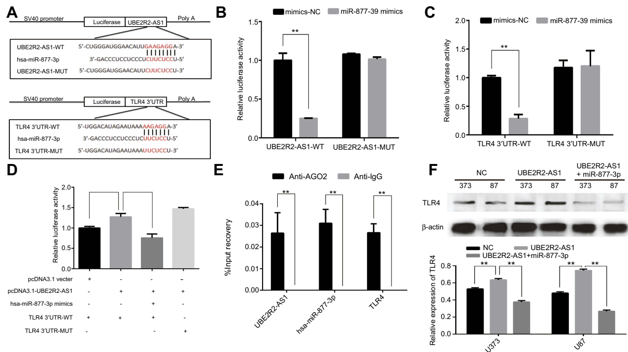
Figure 4 UBE2R2-AS1 is a target of miR-877-3p and regulates the expression of TLR4 as a molecular sponge for miR-877-3p. (A) Bioinformatics predicted miR-877-3p binding sites in UBE2R2-AS1 and TLR4 3'UTR. Mutation was generated on the UBE2R2-AS1 and TLR4 3'UTR sequence in the complementary site for the seed region of miR-877-3p. UBE2R2-AS1 containing wild type or mutant miR-877-3p binding sequence was cloned into psiCHECK-2 luciferase reporter. (B) Luciferase activity was measured in U87 cells co-transfected with wild type (UBE2R2-AS1-WT) or mutant (UBE2R2-AS1-MUT) UBE2R2-AS1 and miR-877-3p using the luciferase reporter assay. (C) Luciferase activity was measured in U87 cells co-transfected with wild type (TLR4 3'UTR-WT) or mutant (TLR4 3'UTR-MUT) TLR4 3'UTR and miR-877-3p using the luciferase reporter assay. (D) TLR4 3'UTR-WT or TLR4 3'UTR-MUT and miR-877-3p constructs were co-transfected into U87 cells with plasmids expressing UBE2R2-AS1 (pcDNA3.1-UBE2R2-AS1) or with a control vector to verify the ceRNA activity of UBE2R2-AS1. Luciferase activity was measured in U87 cells 48 h after transfection. (E) RIP with mouse monoclonal anti-Ago2, preimmune IgG or input from U87 cells extracts. RNA levels in immunoprecipitates were determined by qRT-PCR. Levels of UBE2R2-AS1, miR-877-3p and TLR4 RNA were presented as percentages input recovery in Ago2 relative to IgG immunoprecipitates. (F) Western blot analysis of TLR4 protein level following treatment of U87 cells and U373 cells with pcDNA3.1-UBE2R2-AS1 and miR-877-3p mimics. β-actin was used as control.
