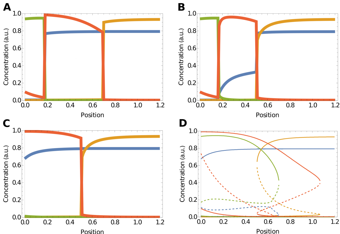
Fig 5. Olig2 repression of Pax6 increases robustness to initial conditions. (A) Patterning without the repressive link from Olig2 to Pax6, showing steady states reached from standard initial conditions. Compared to the full network, the qualitative domain structure is conserved. (B) Patterning for the full network for initial conditions with high levels of Pax6 and Irx3 is qualitatively identical to low initial levels of Pax6 and Irx3. Initial conditions [Pax6] = [Irx3] = 1. (C) Patterning without the repressive link from Olig2 to Pax6 for initial conditions with high levels of Pax6 and Irx3. The p3 domain is lost as a consequence of the different initial conditions. (D) Bifurcation diagram of the network without Olig2-Pax6 repression. The region in which the pMN state (Olig2 high) is stable has expanded ventrally, thus making the ventralmost region bistable.
