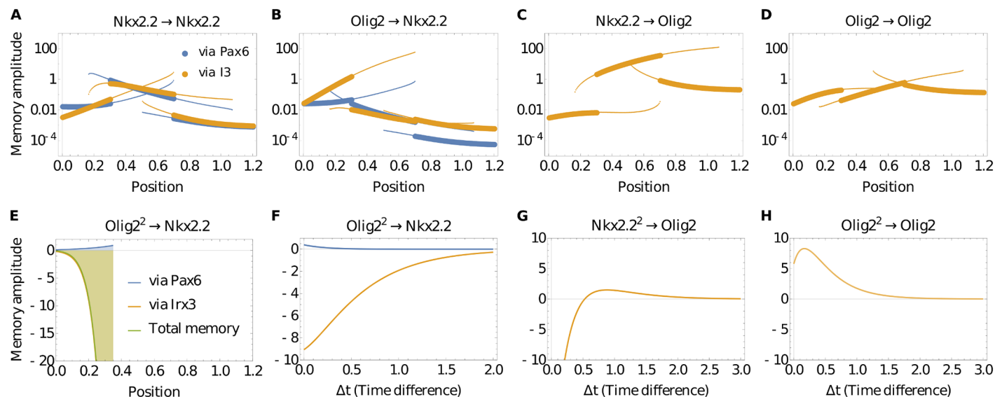
Fig 4. Memory amplitude and temporal dynamics. (A) Amplitude of memory (memory function at \Delta t = 0 ) of Nkx2.2 to itself along the neural tube. There are multiple lines as the analysis was performed at all possible stable steady states. The vertical axis is logarithmic to make the range of amplitudes easier to appreciate. Colours identify the memory amplitude contribution from each of the two possible bulk channels, via Irx3 and Pax6, respectively. Thick lines indicate physiological states, while thin lines indicate states that are not usually observed in vivo. (B) Linear memory amplitude of (past) Olig2 on Nkx2.2 along the neural tube. The memory via Pax6 is for the most part below the memory via Irx3 in each pair of corresponding curves. (C,D) Memory amplitudes of Olig2 to Nkx2.2 (C) and to itself (D). No channel decomposition is performed as Olig2 receives memory only via the Irx3 channel. (E) Nonlinear memory function of (past) Olig2 squared on Nkx2.2 in the p3 domain, where dynamics are dominated by Irx3; memory via Pax6 is negligible by comparison. (F) Nonlinear memory function of (past) Olig2 squared on Nkx2.2 from position 0.2 in (E), plotted to show that the relative contribution of the Pax6 channel is small also for all time differences. (G,H) Nonlinear memory functions of Olig2 to Nkx2.2 (G) and itself (H) in the p2 domain at position 0.7, exemplifying the potential for nontrivial time dependences (including non-monotonicity and sign changes) in the nonlinear memory functions.
