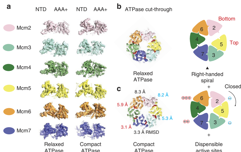
Figure 3 | The MCM ATPase centres. (a) Segmented density and docked atomic structures of the six Mcm2-7 protomers in the two conformers. The NTD and AAA+ domains tilt and rock with respect to one another. (b) ATPase sites in the relaxed ATPase conformer. (c) ATPase sites in the compact ATPase conformer. One side of the MCM ring is more static and the corresponding active sites are dispensable for viability (– means Walker A mutation kills DNA unwinding, + means tolerated mutation).
