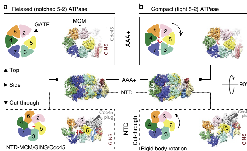
Figure 2 | Two configurations in the ATPγS-CMG-DNA complex. (a) AAA +, side and cut-through view of the CMG in a relaxed ATPase configuration. Cdc45 topologically locks the Mcm5-2 gate. (b) AAA +, side and cut-through N-terminal view of the CMG in a compact ATPase configuration. DNA density surmounting the AAA + domain has been removed for visualization purposes (also see Fig. 4).
