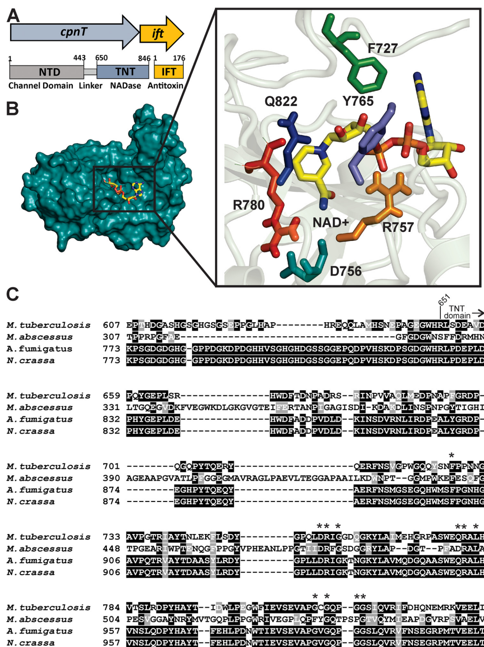
Figure 1. TNT family enzymes contain conserved catalytic residues. A, the cpnT-ift operon of M. tuberculosis and the domain organization of CpnT. B, putative NAD + -binding site of TNT in the docking model (18) with conserved residues highlighted. C, alignment of TNT homologs in mycobacteria and fungi. All sequences were obtained from Pfam: Pf14021. The sequence alignment was visualized using the T-Coffee and BoxShade servers.
