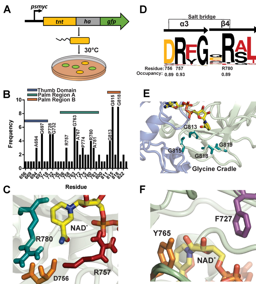
Figure 5. Selection of nontoxic TNT mutants in E. coli . A , scheme of the reporter selection screen. Green colonies indicate E. coli clones expressing full-length tnt – gfp mutants with reduced toxicity. B , number of mutants obtained at the indicated residue and the relative location within the TNT structure. C , potential DRXG–QRXL salt bridge in the predicted NAD + -binding site. D , the relative occupancy and residue number of the DRXG and QRXL motifs in CpnT obtained from the hidden Markov model using the TNT family of proteins and modeled using Skyline and WebLogo. E , glycine cradle located at the base of the NAD + -binding site predicted by the docking model. F , Tyr 765 and Phe 727 are located close to the nicotinamide moiety in the predicted NAD + -binding site.
