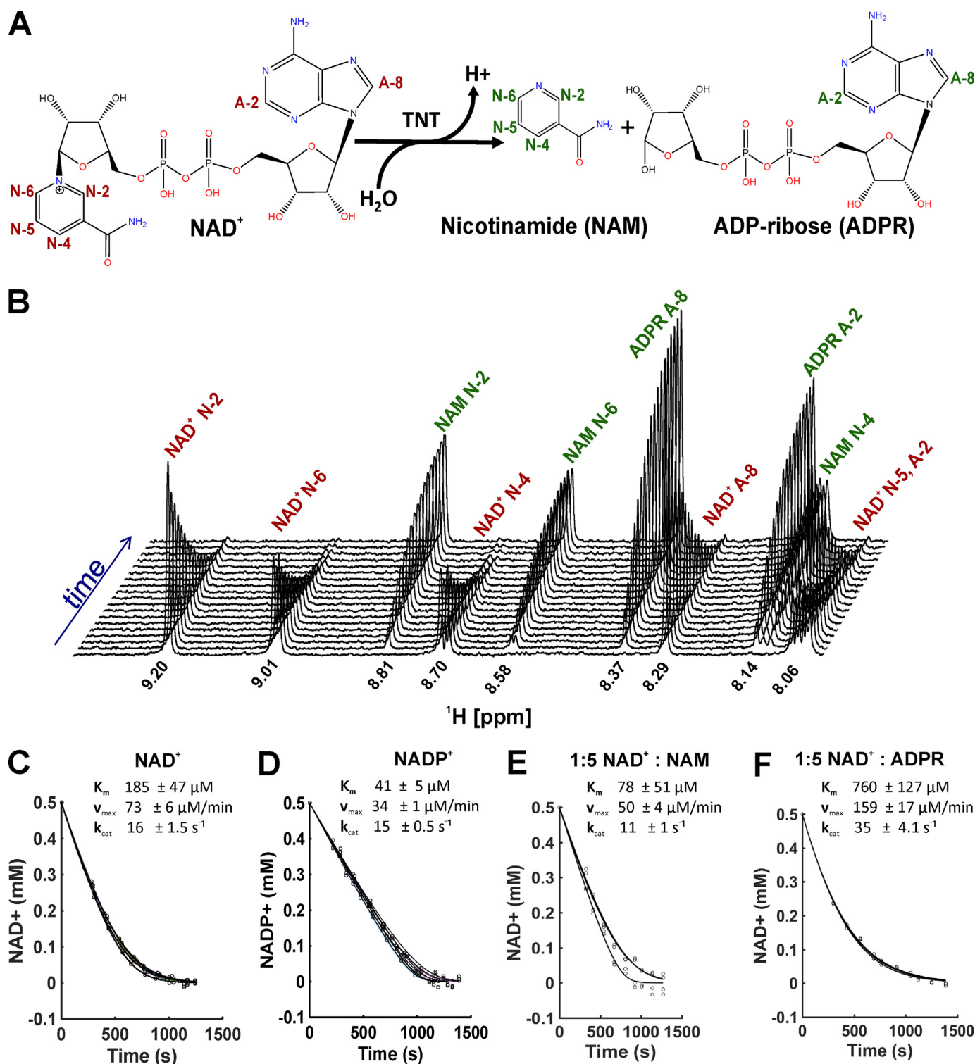
Figure 3. Kinetic analysis of TNT substrate hydrolysis and inhibition. A, NAD + hydrolysis by TNT. N and A indicate protons from nicotinamide and adenine, respectively. Red indicates signals corresponding to NAD + , whereas green represents signals from hydrolyzed products. B, time course of NAD + hydrolysis and nicotinamide and ADP-ribose formation as followed by 1 H NMR. Chemical shifts and assignments of the signals are indicated. C, NAD + (500 \mu M) hydrolysis by 75 nM TNT and average kinetic parameters ( n = 3 ). The signal intensities corresponding to NAD + N-2, N-4, and N-6 were plotted and used for curve fitting in C and D. D, NADP + (500 \mu M) hydrolysis by 37.5 nM TNT and average kinetic parameters ( n = 3 ). E, NAD + (500 \mu M) hydrolysis kinetics in the presence of 75 nM TNT and 2.5 mM nicotinamide ( n = 2 ). The signal intensities corresponding to NAD + N-2 and N-6 were plotted and used for curve fitting in E and F. F, NAD + (500 \mu M) hydrolysis kinetics in the presence of 75 nM TNT and 2.5 mM ADP-ribose ( n = 3 ).
