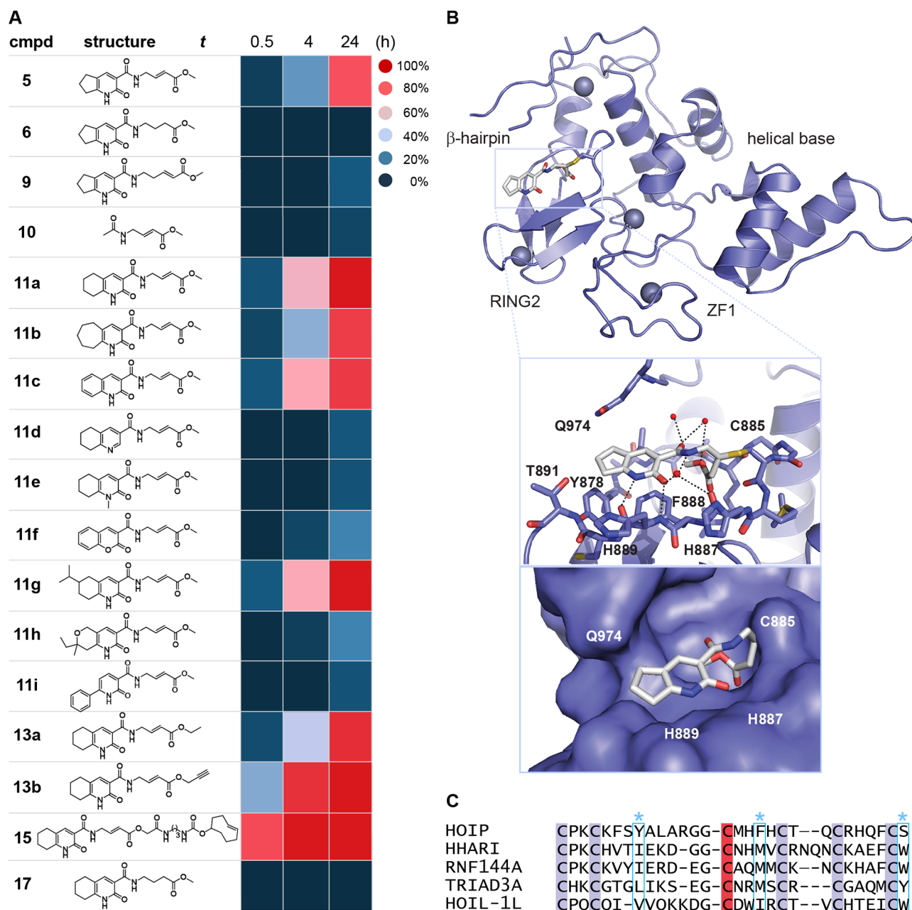
Figure 5. Molecular determinants for interactions between the HOIP RING2 domain and compound (5). (A) LC–MS screening data plotted as percentage labeling of the HOIP RBR domain (2 \mu M) by key analogues (6), (9)–(11), (13), (15) (20 \mu M), and (17) (200 \mu M) after 0.5, 4, and 24 h incubation. For full screening data see SI Figures S7 and S8. (B) Ribbon representation of the HOIP RING2-LDD domain structure in complex with compound (5) at 2.15 Å resolution (PDB: 6GZY). Zn 2+ ions are shown as gray spheres and compound (5) as ball and stick. The inset shows a zoom into the active site showing hydrogen bonds (dashed lines) made by compound (5) with water molecules (red spheres) and HOIP (top), and the pocket around the active site which accommodates compound (5) (bottom). (C) Sequence alignment of RING2 domains of those RBR E3 ligases that were screened against compound (5). The catalytic cysteine residue is highlighted in red, noncatalytic cysteine residues in purple, and nonconserved residues contributing to the compound-binding pocket in HOIP are highlighted with a blue asterisk.
